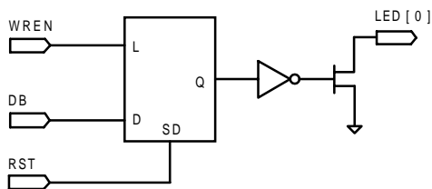
Figure 10.1. LED0 Port Structure
