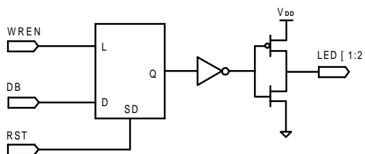
Figure 10.2. LED1, LED2 Port Structures
